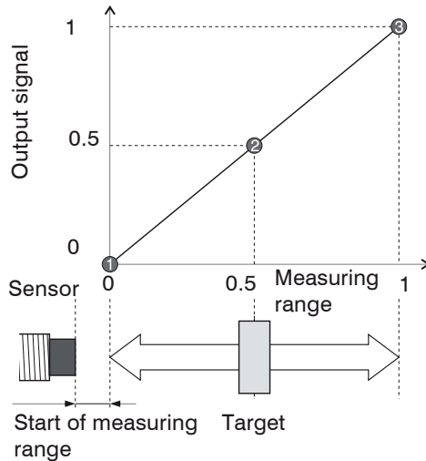
Fig. 19 Calibration steps
