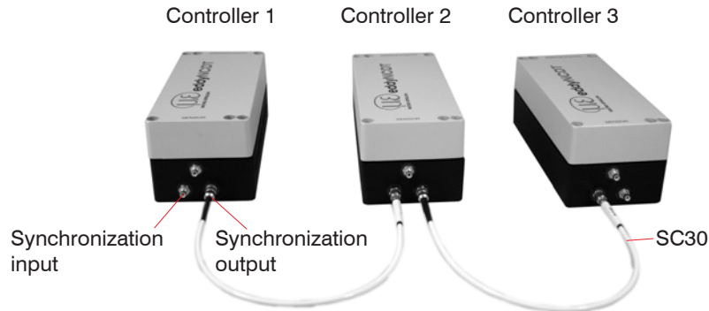
Fig. 8 Synchronized multichannel measuring system
