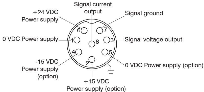
Fig. 14 Socket pin assignment and signal output for standard supply (+24 VDC) and optional supply ( \pm 15 VDC) - view on solder pin side female cable connector
