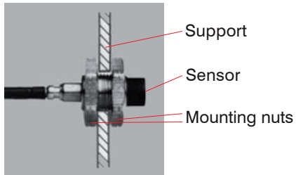
Fig. 9 Unshielded sensor with thread in standard mounting
