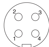
Fig. 6 4-pin male cable connector, solder side view
