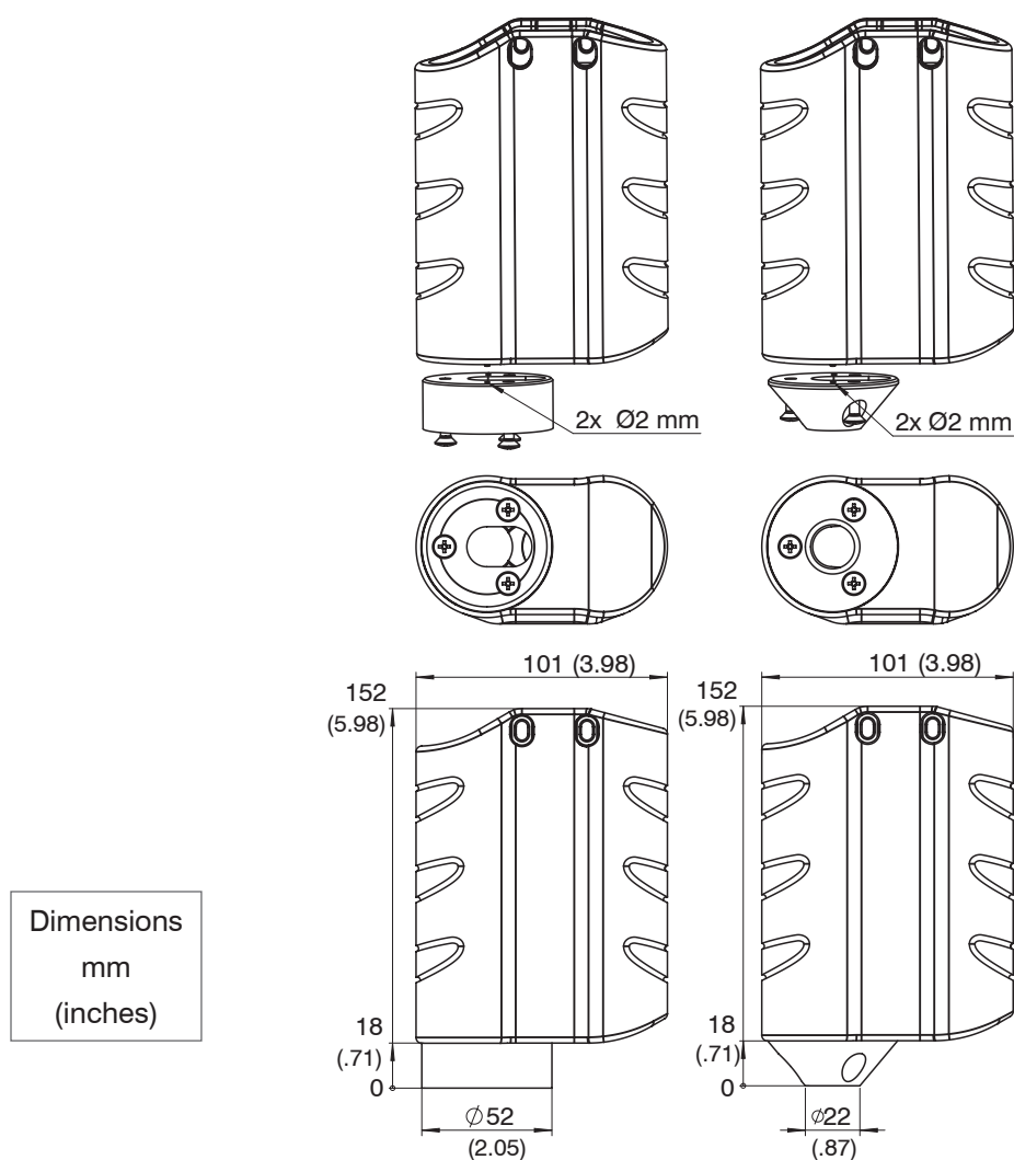
Fig. 25 FCS-X-ACS1-30/0-50-XXXX angle sensor adapter
