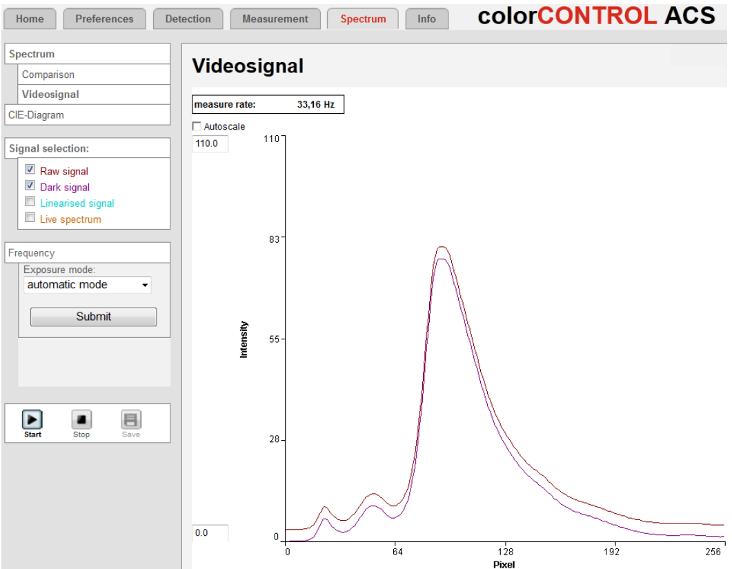
Fig. 45 Video Signal program
