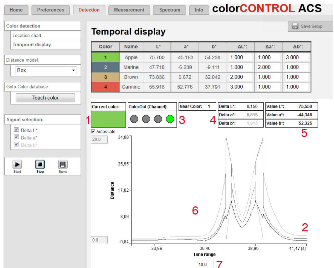
Fig. 39 Time diagram program
