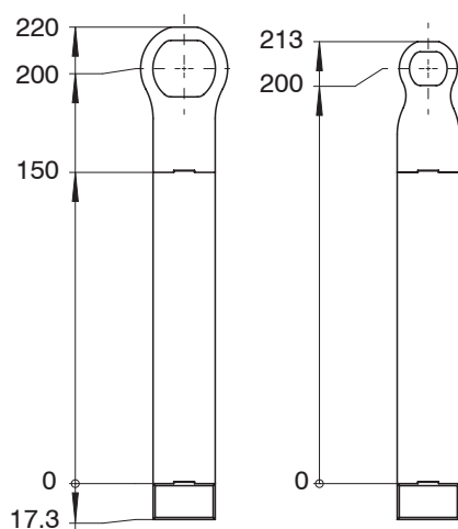
Fig. 23 FCS-ACS3, mounting adapter 150 mm
