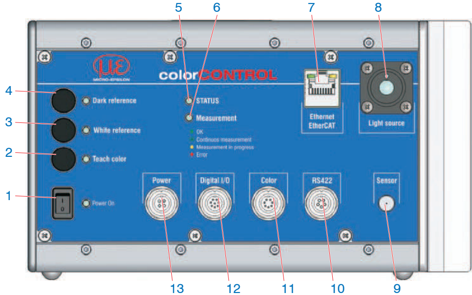
Fig. 3 Controller front view
