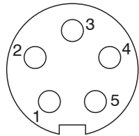
Fig. 12 5-pin male cable connector, solder side view
